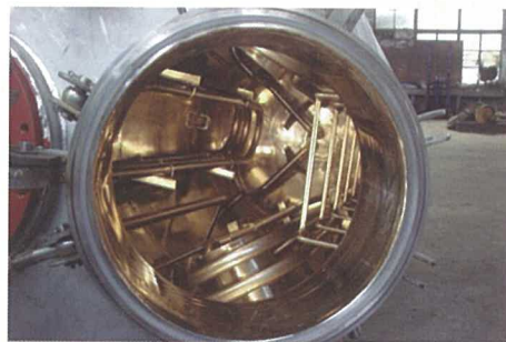
种子罐内部结构图 inner structure illustration of seeding tank
